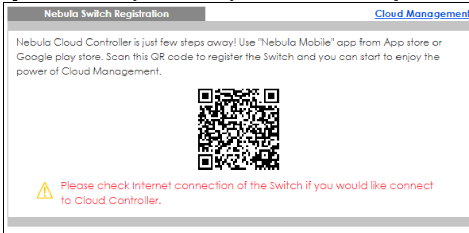
Figure 84 Basic Setting > Cloud Management > Nebula Switch Registration
