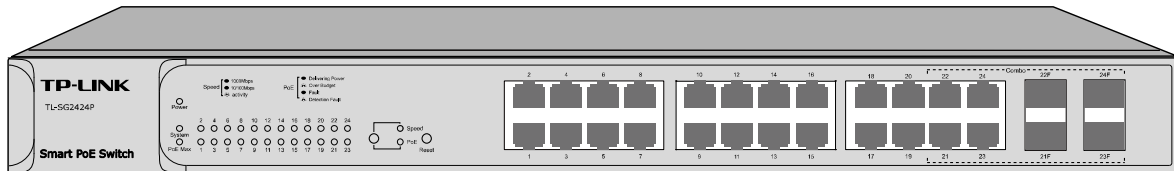
Figure 2-3 Front Panel of TL-SG2424P
