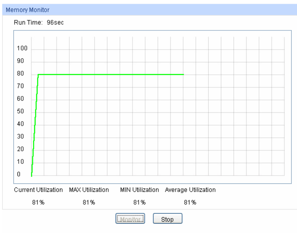
Figure 14-2 Memory Monitor
