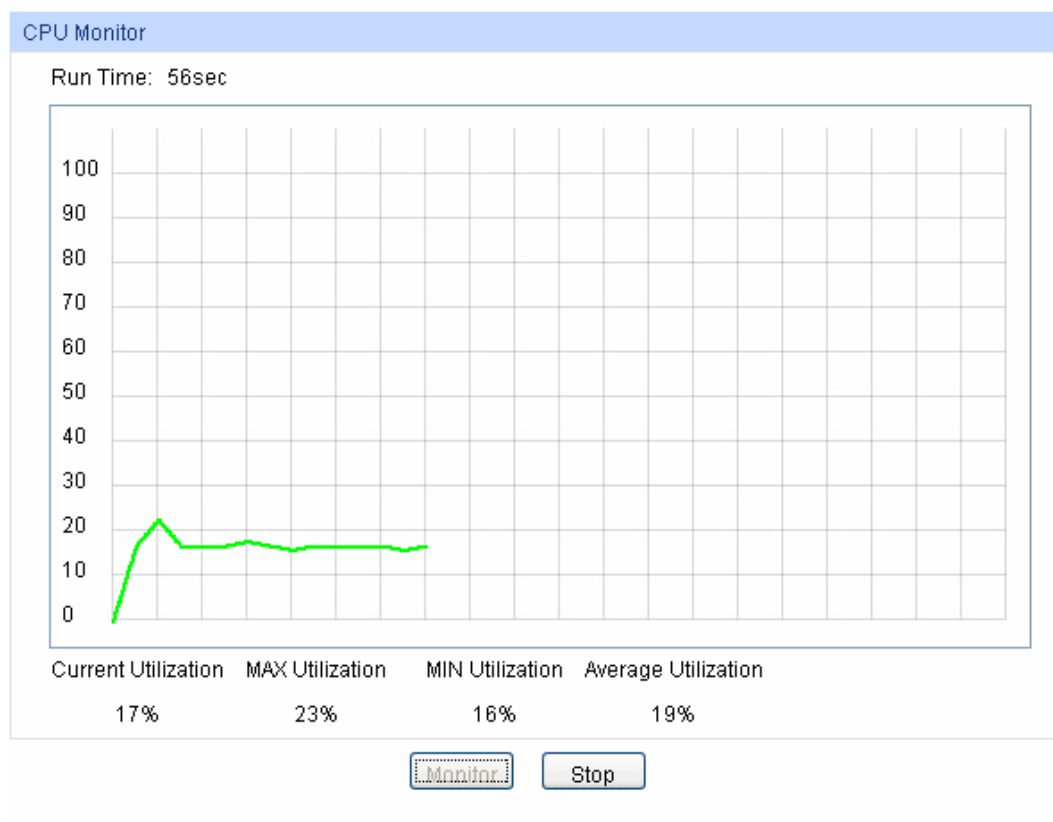
Figure 14-1 CPU Monitor
