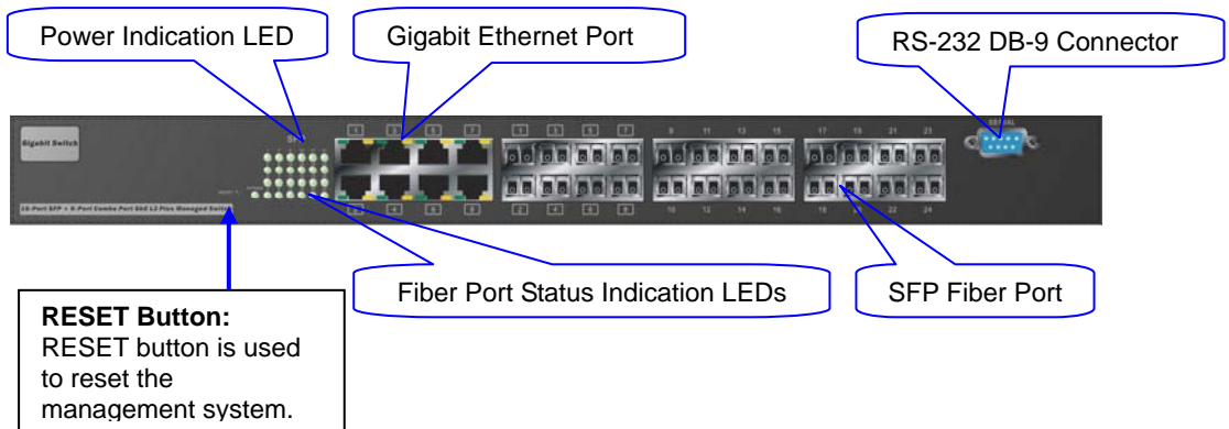
Fig. 1-2 Front View of GEFXL2P-SW24
